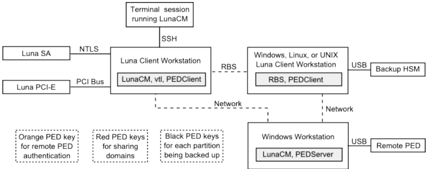
Figure 2: Configuration for remote backup of a SafeNet HSM client workstation slot with the remote PED connected to a separate workstation
